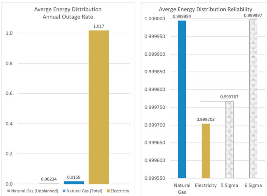
Figure 44: Natural Gas and Electric Distribution Outage Rates and Service Reliability
