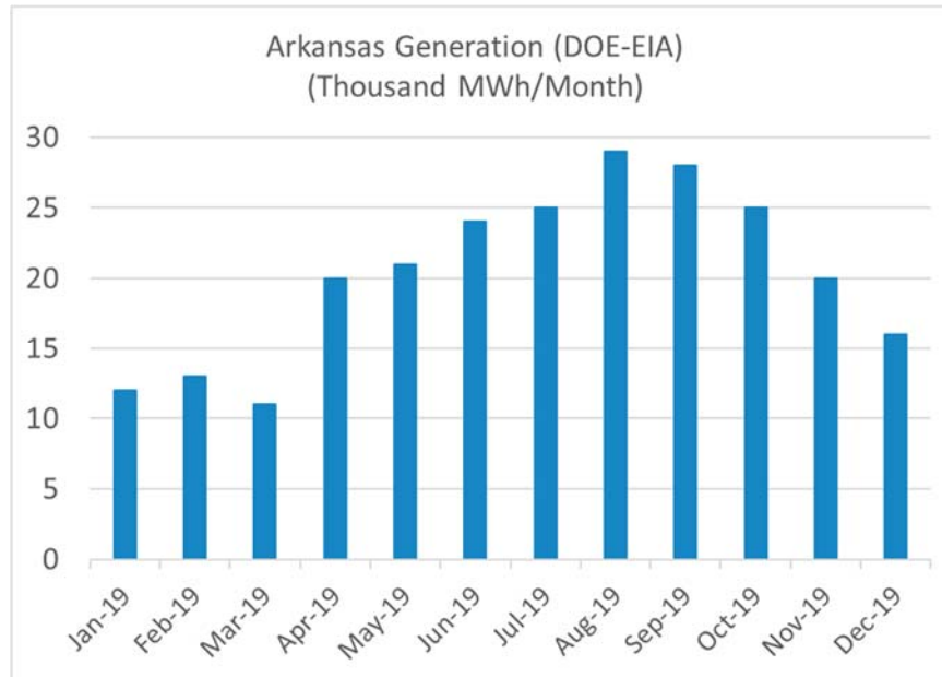
Figure 26: Monthly Arkansas Solar PV Generation (DOE-EIA)
