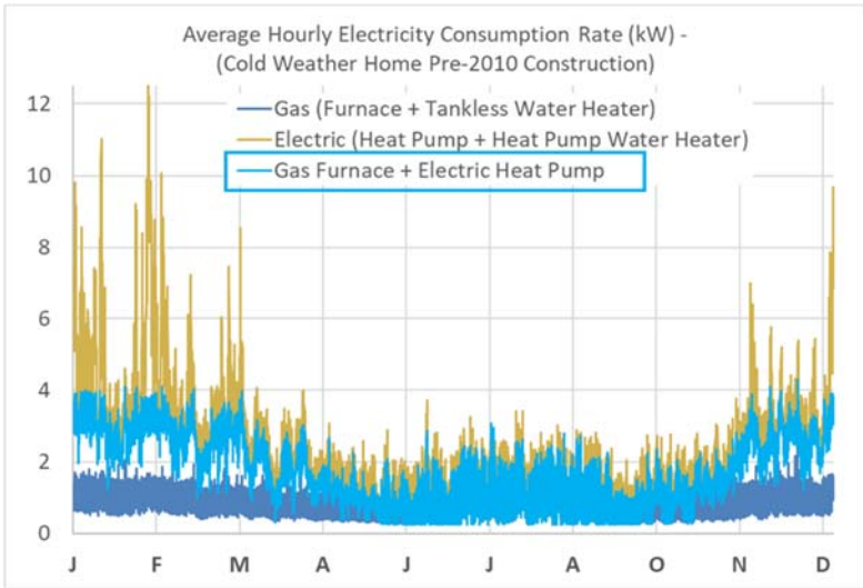
Figure 19: Hybrid Natural Gas and Electric Space Heating System (GTI)
