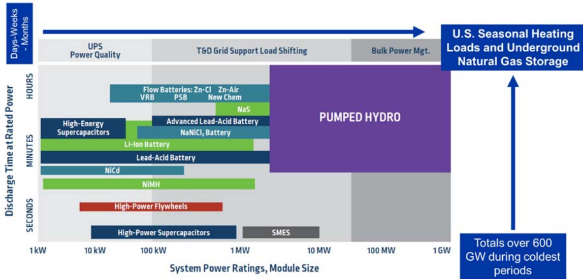
Figure 42: Size and Duration of Energy Storage Systems (adapted from National Hydropower Association report)
