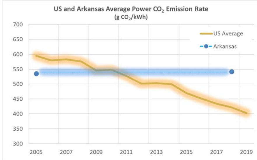
Figure 23: US Power Generation Average CO 2 Emission Rate (DOE-EIA)
