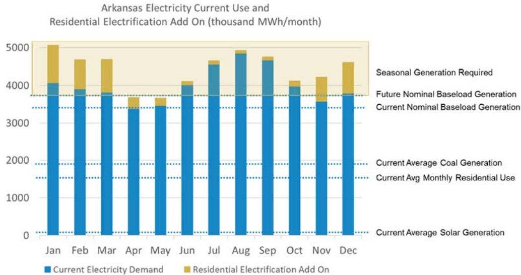
Figure 27: Arkansas Current Monthly Electricity Use and Projected Impact of Full Residential Electrification
