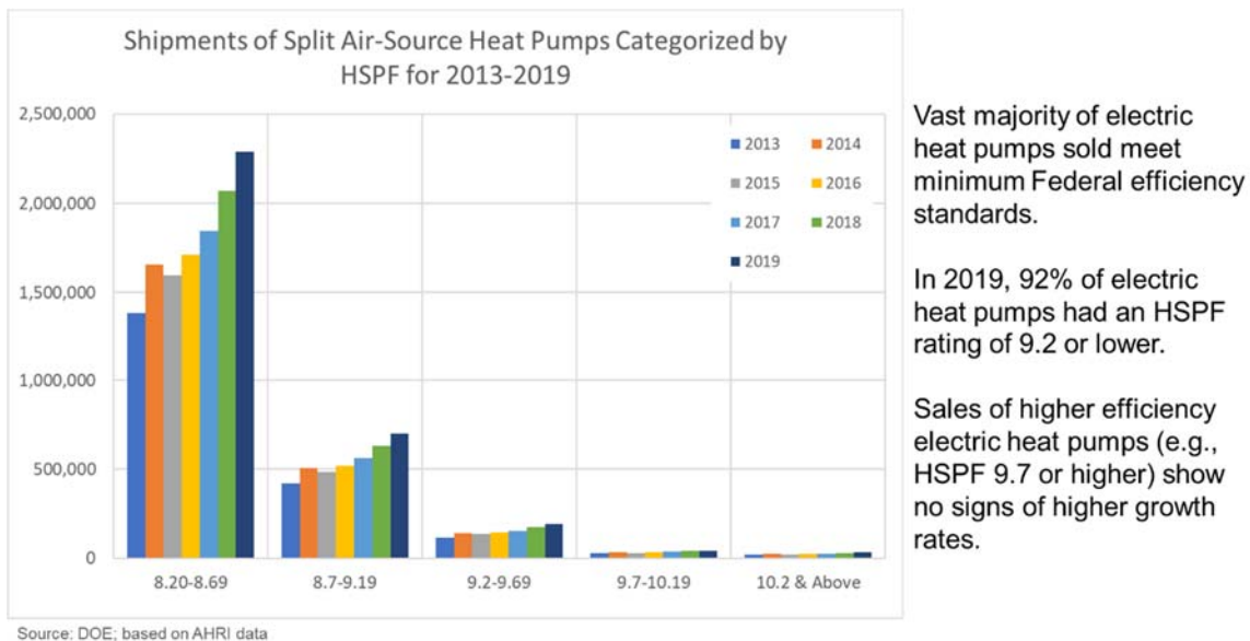
Figure 12: Residential Electric Air-Source Heat Pumps Sales Estimates
