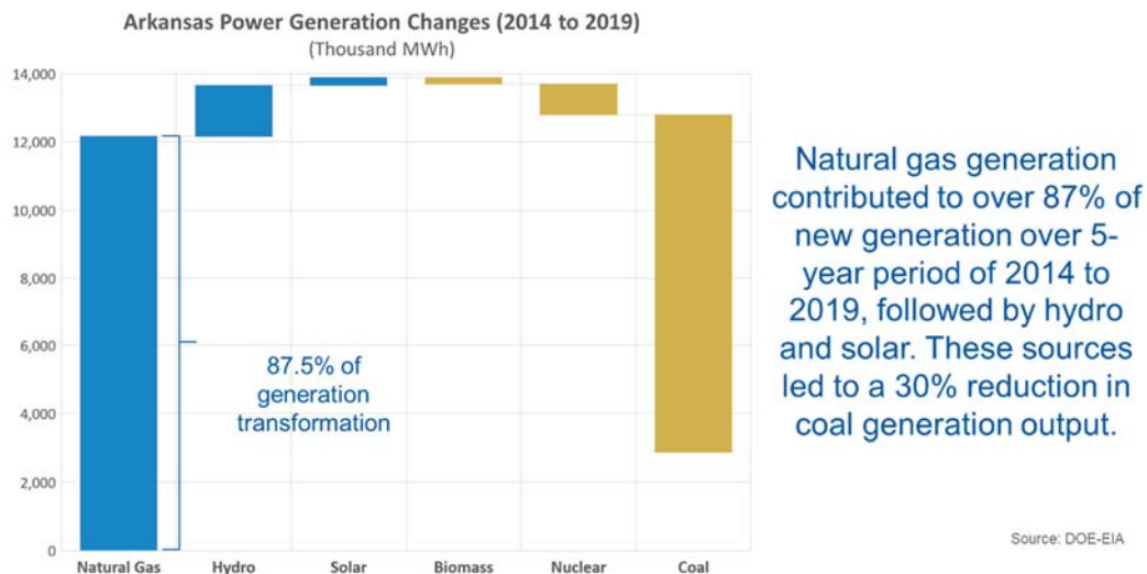
Figure 22: Arkansas Power Generation Changes (2014–2019, DOE-EIA)
