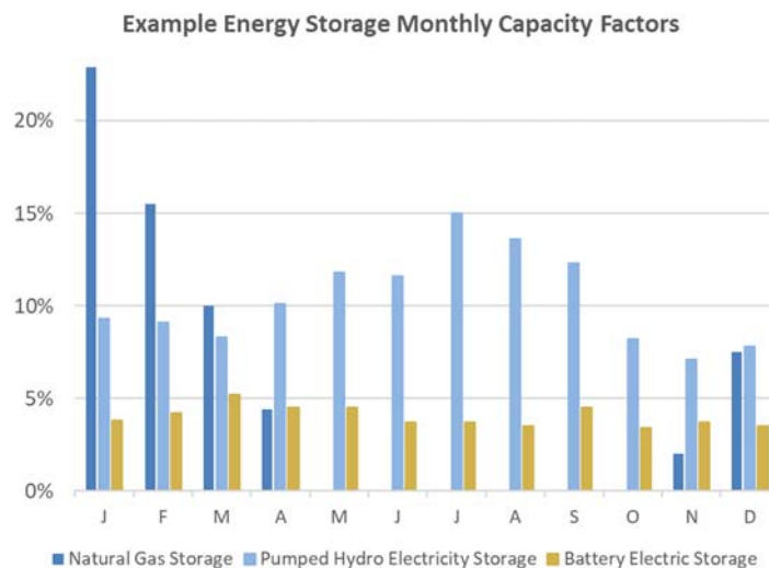
Figure 41: Example Energy Storage System Capacity Factors (DOE-EIA)
