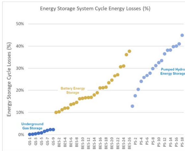
Figure 40: Energy Storage Cycle Energy Losses (DOE-EIA, GTI)
