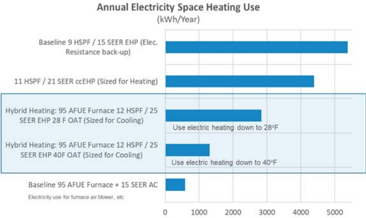
Figure 20: Hybrid Natural Gas and Electric Heating System Comparisons (GTI)
