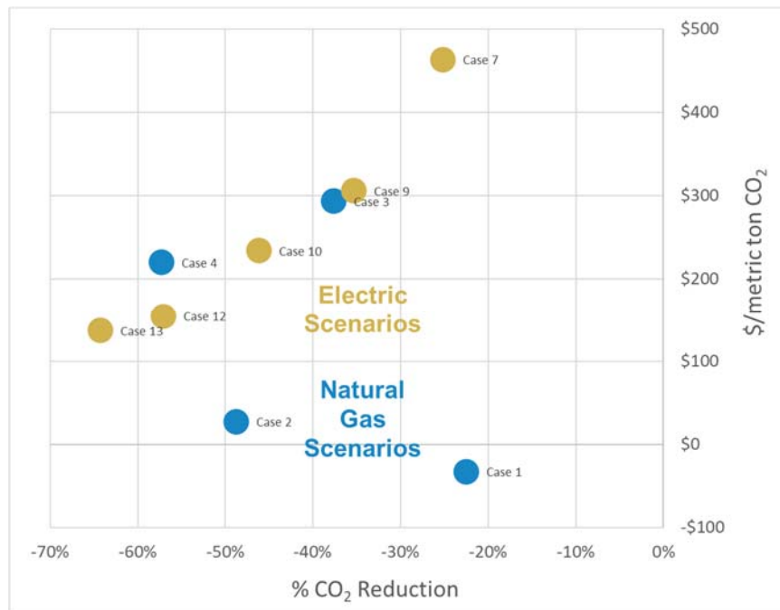
Figure 33: Fayetteville, AR Residential GHG Reduction Scenarios
