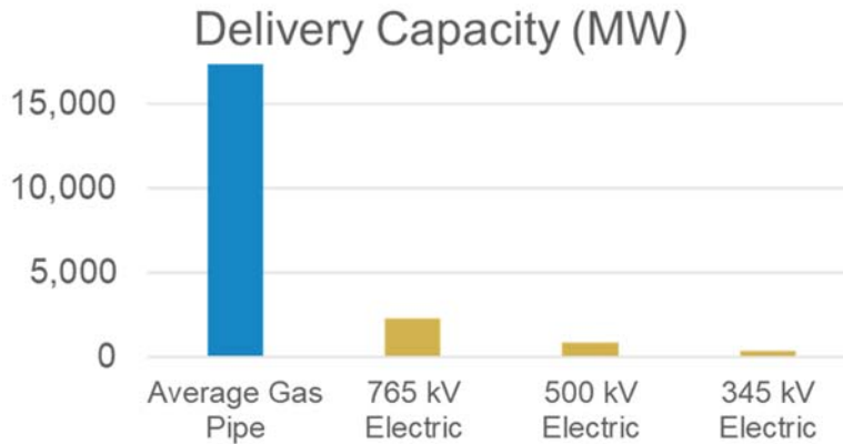
Figure 37: Major Natural Gas and Electric Transmission System Capacity (DOE, AEP)
